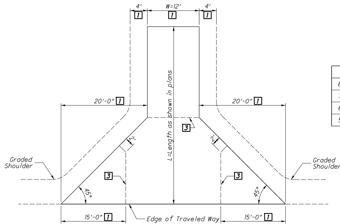
TYPE 2 DRIVEWAY
